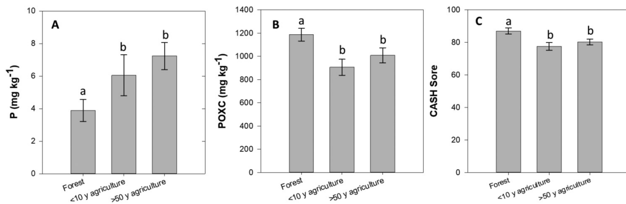
Fig. 4. (A) Concentrations of phosphorus, (B) permanganate oxidizable carbon (POXC), and (C) Comprehensive Assessment of Soil Health (CASH) scores in mineral soils (0–15 cm) collected at forest sites and <10- and >50-year agricultural sites. Bars are mean \pm standard error. Significant differences ( p < 0.05 ) are denoted by different letters.
